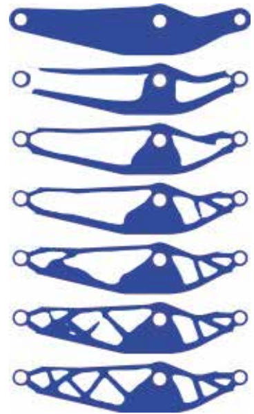
Optimisation sequence for plastic bracket in OptiStruct
